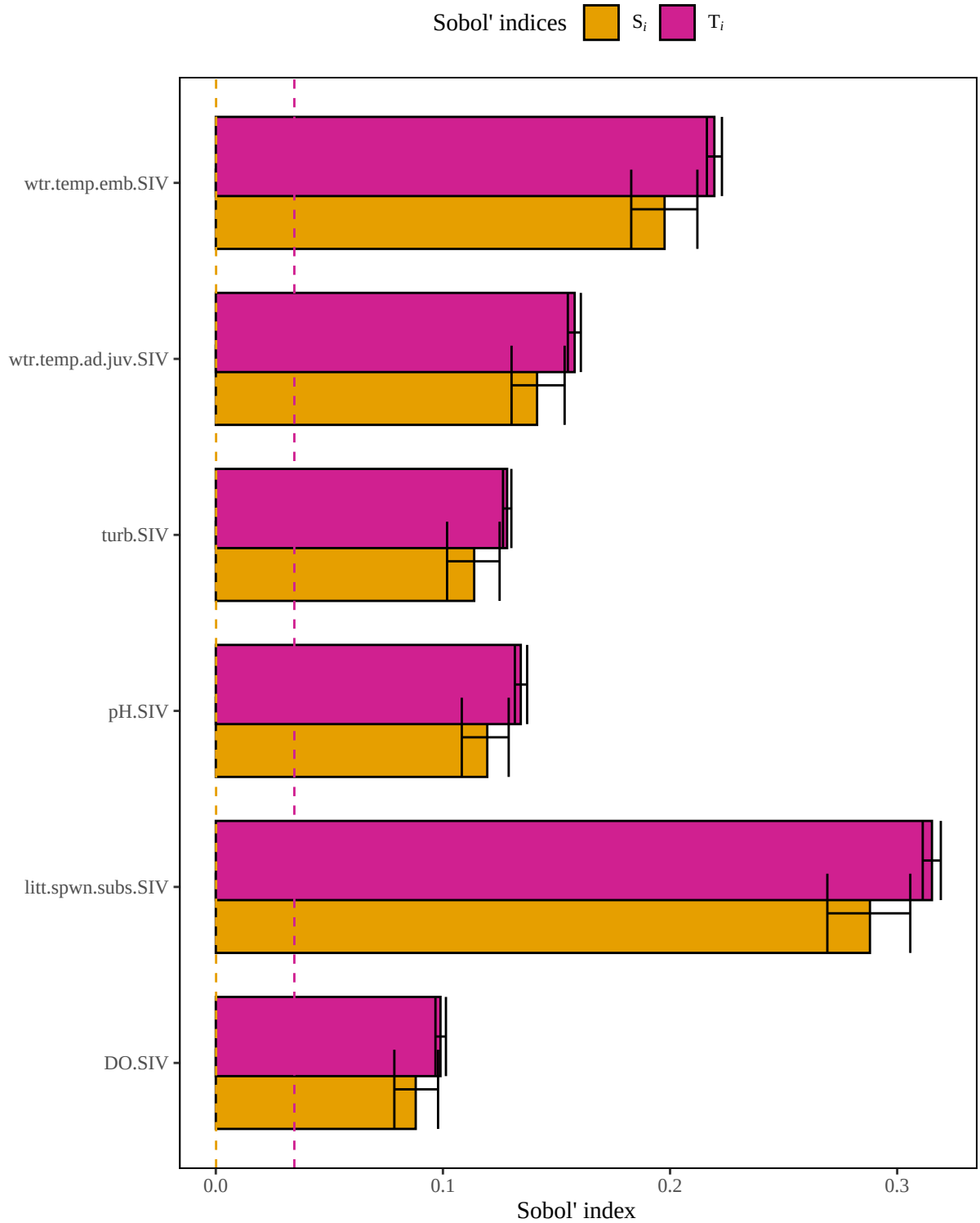
Figure 5. Results of a sensitivity analysis for the whitesuckerLacSpwnLakeDrawMtoe2m model based on a geometric mean structure. Dashed lines represent baseline numerical approximation error for S_i and T_i ( i.e. , dummy variables).
